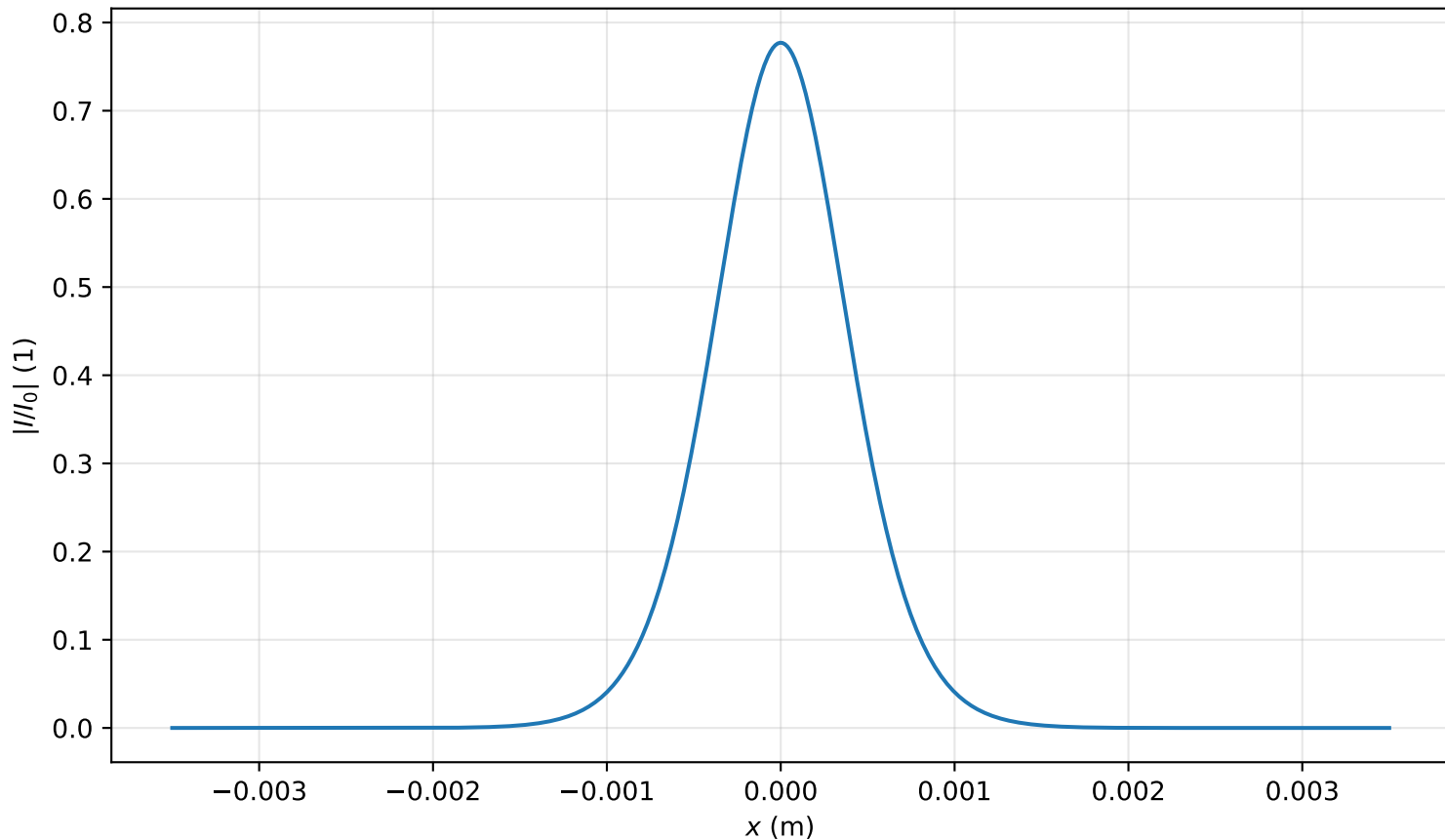
Intensity profile I(x, y = 0, z = 1.831m)/I_0 , P_{in}=0.4P_{cr} , artificial time
